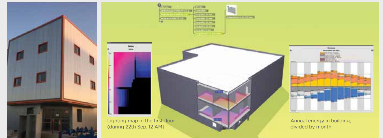
Office building, Israel | Light Simulation
